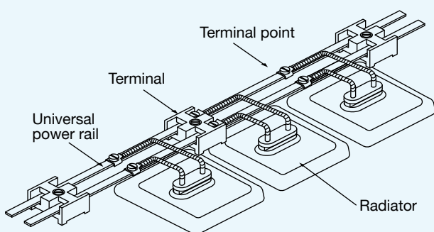
Figure 13: Rail wiring
